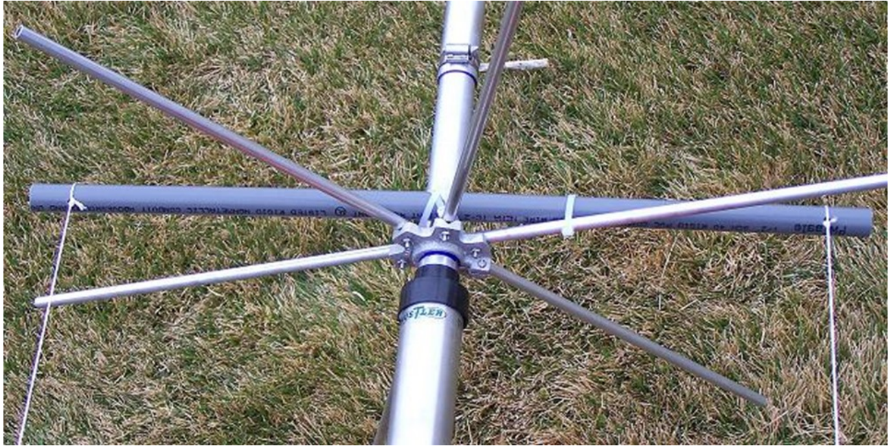
"Top Hat" assembly with cross arm showing support attachments for verticals.
