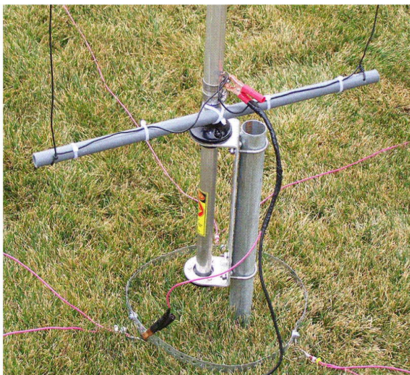
Bottom showing PVC cross arm support with 12 and 17 meter vertical wires attached and connections to radial ring.
